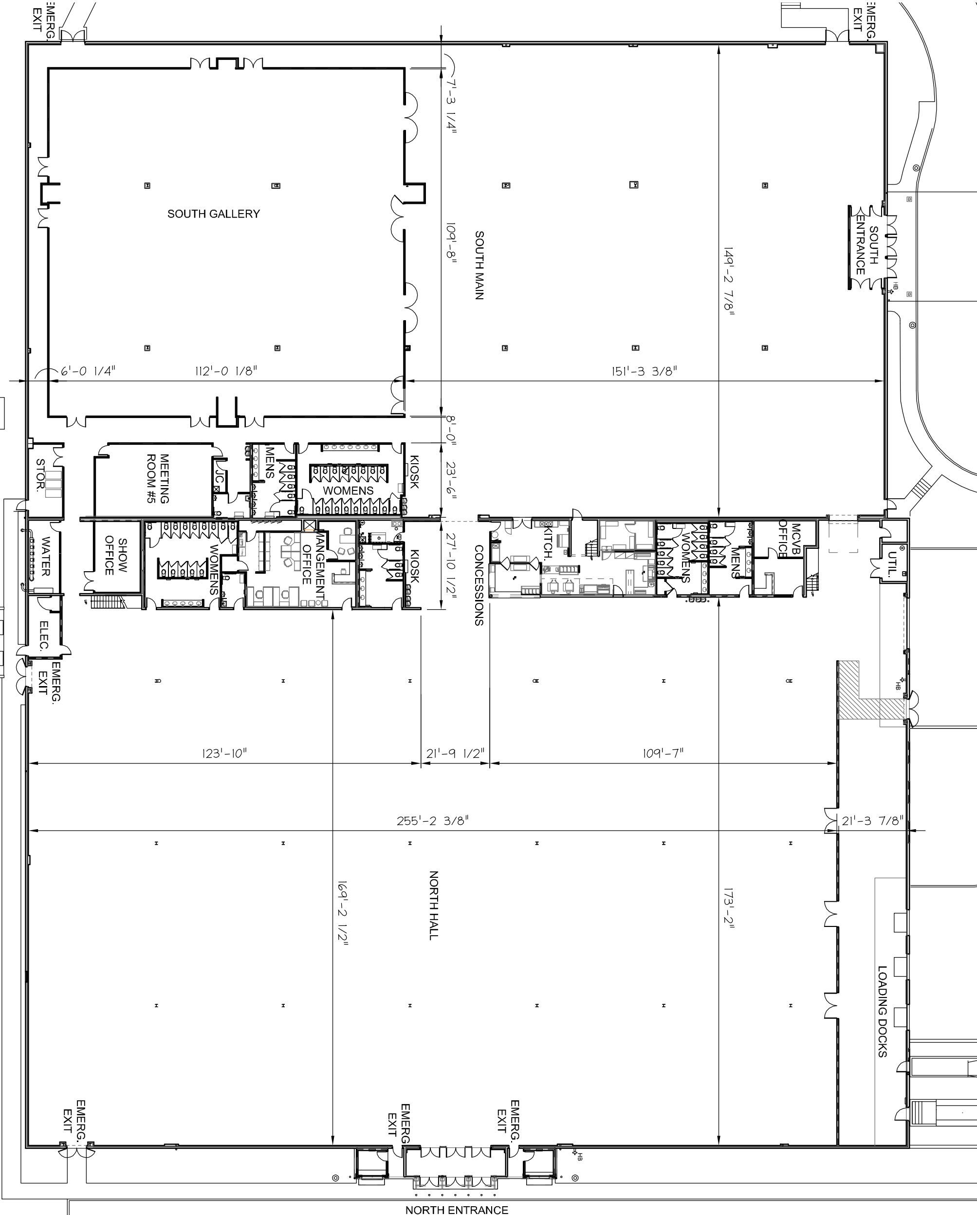
Dimensioned Plan
